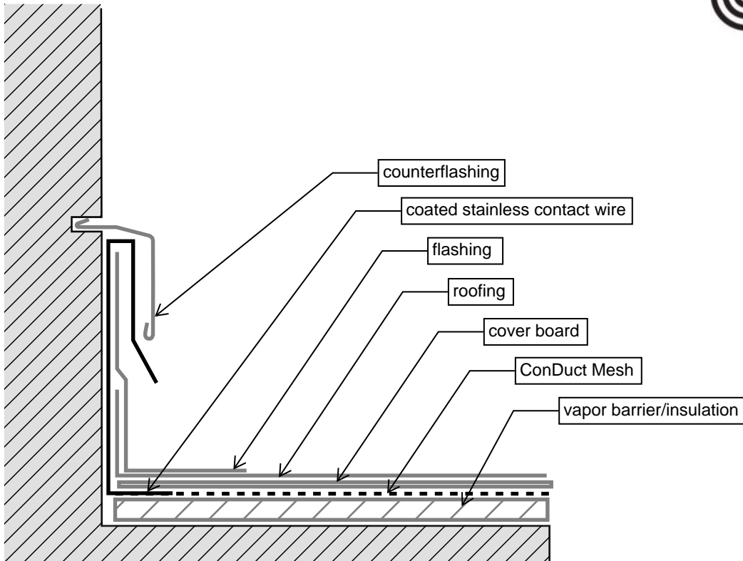
lead wire runs behind the wall and exits at the counterflashing
